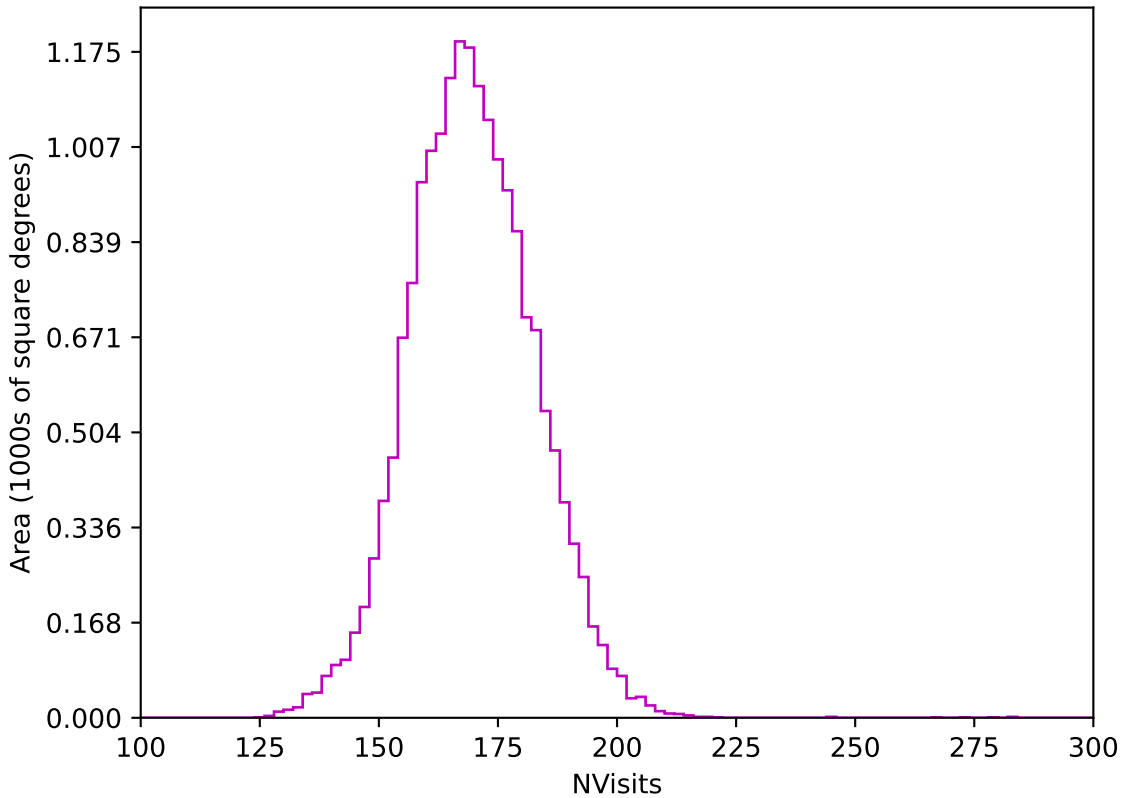
start_date_do-180v3.4_10yrs WFD z band: NVisits
