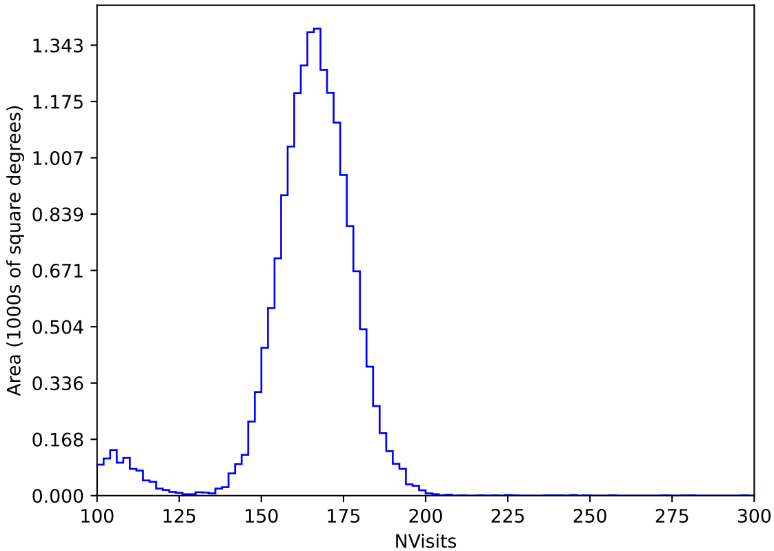
start_date_do-180v3.4_10yrs WFD y band: NVisits
