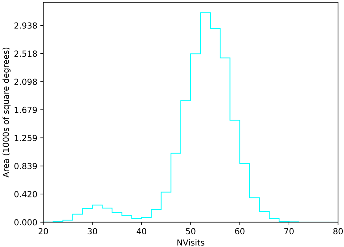
start_date_do-180v3.4_10yrs WFD u band: NVisits
