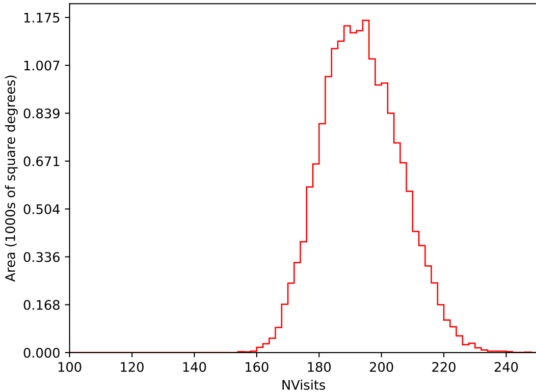
start_date_do-180v3.4_10yrs WFD i band: NVisits
