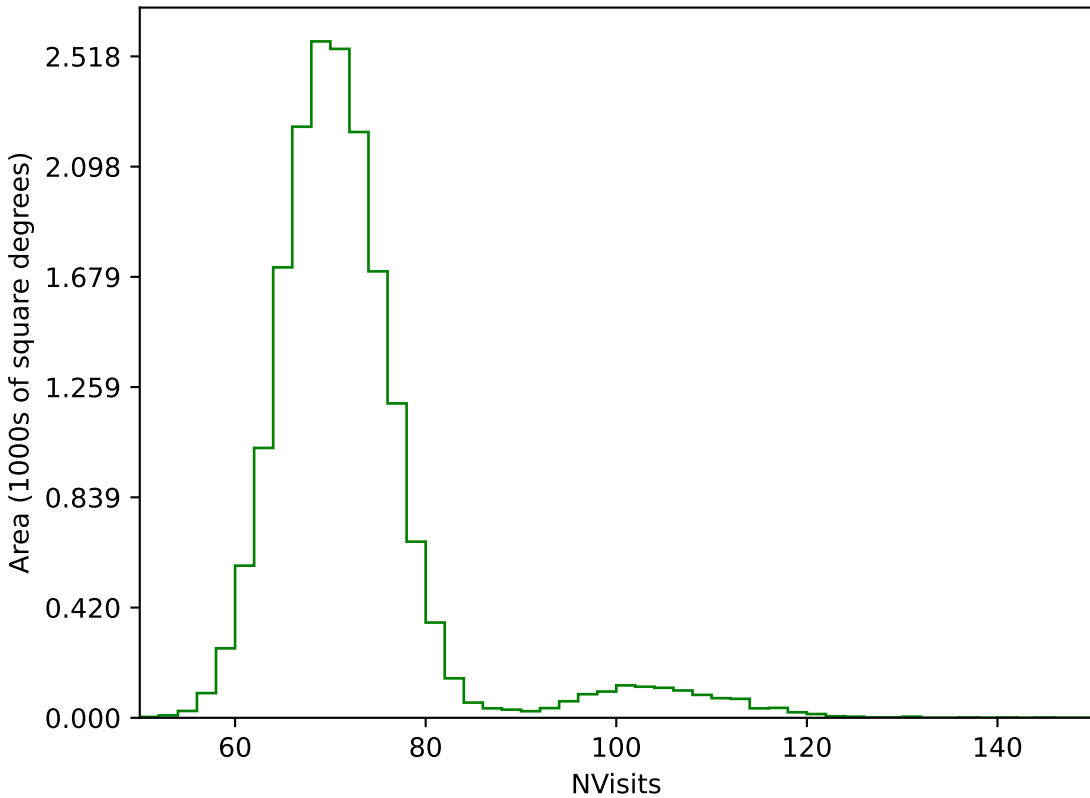
start_date_do-180v3.4_10yrs WFD g band: NVisits
