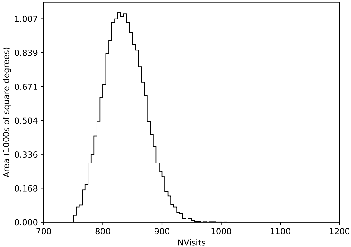
start_date_do-180v3.4_10yrs WFD all bands: NVisits
