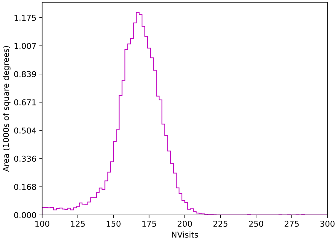
start_date_do-180v3.4_10yrs All sky z band: NVisits
