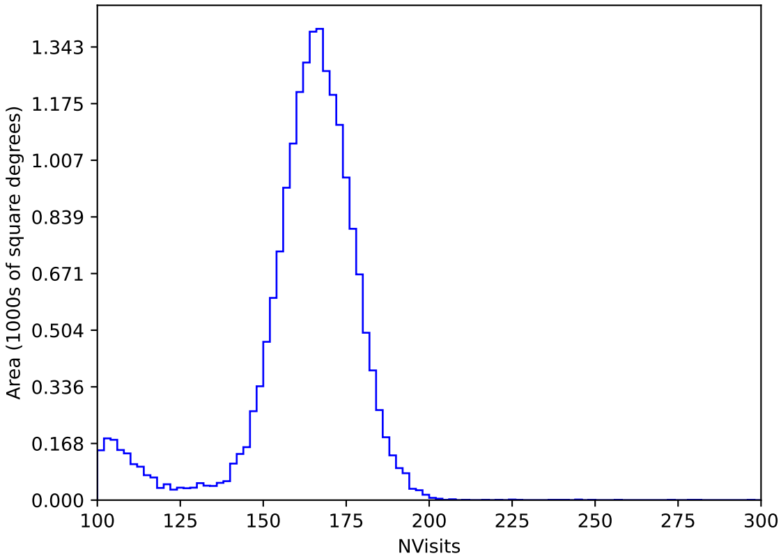
start_date_do-180v3.4_10yrs All sky y band: NVisits
