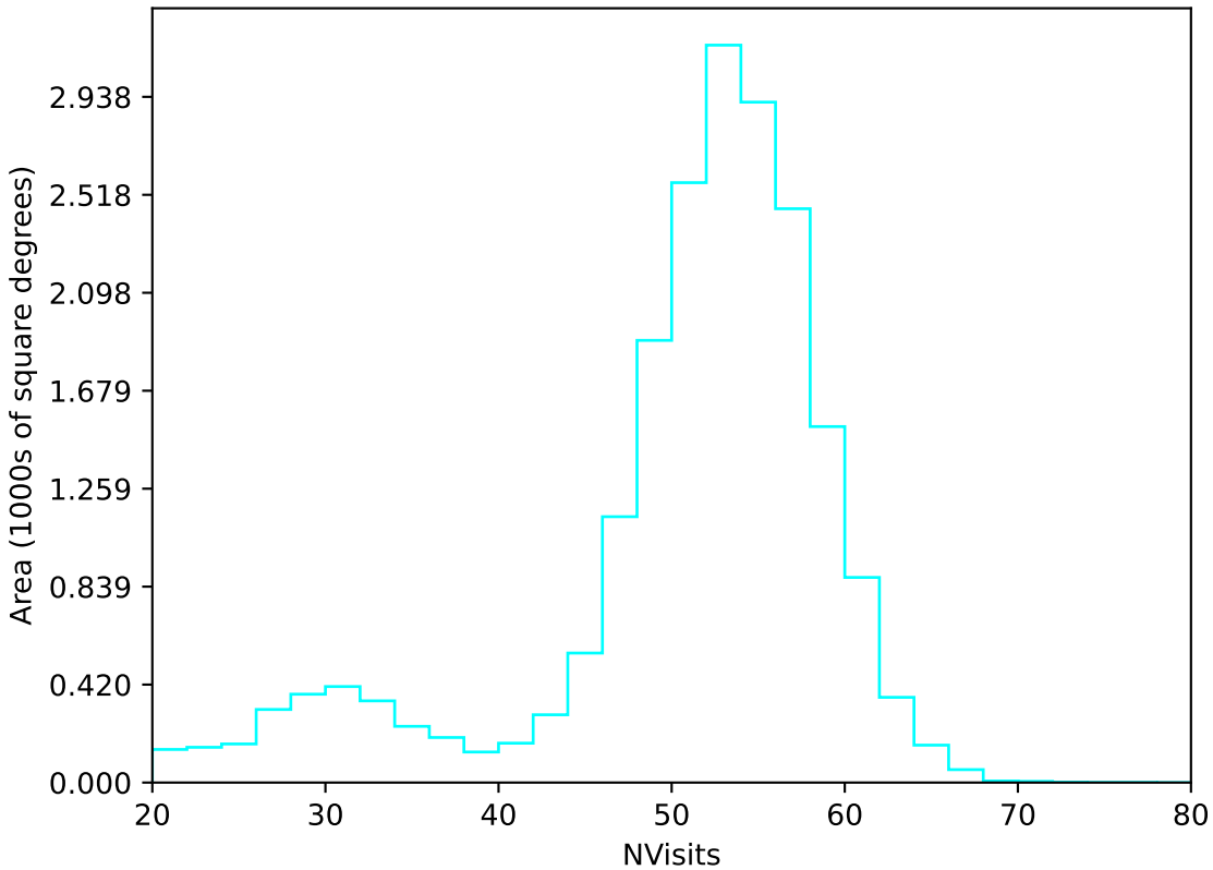
start_date_do-180v3.4_10yrs All sky u band: NVisits
