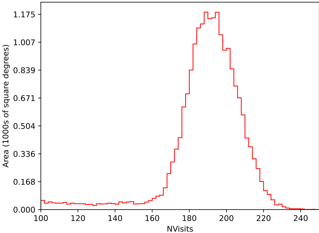
start_date_do-180v3.4_10yrs All sky i band: NVisits
