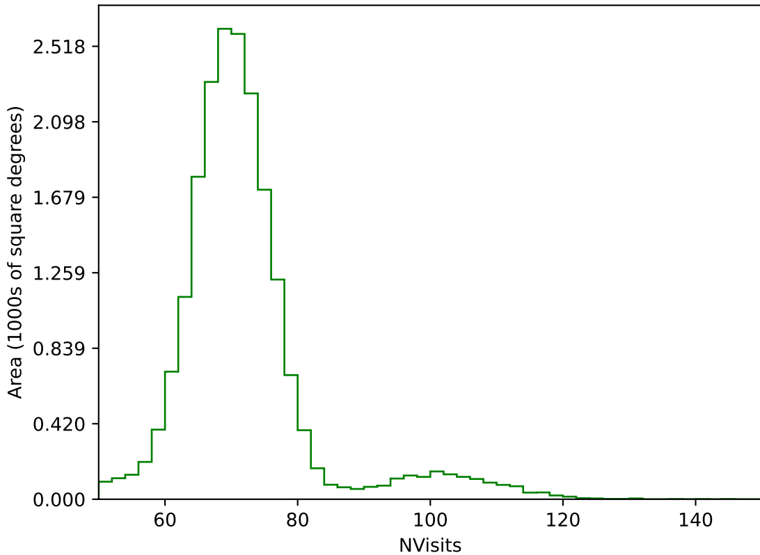
start_date_do-180v3.4_10yrs All sky g band: NVisits
