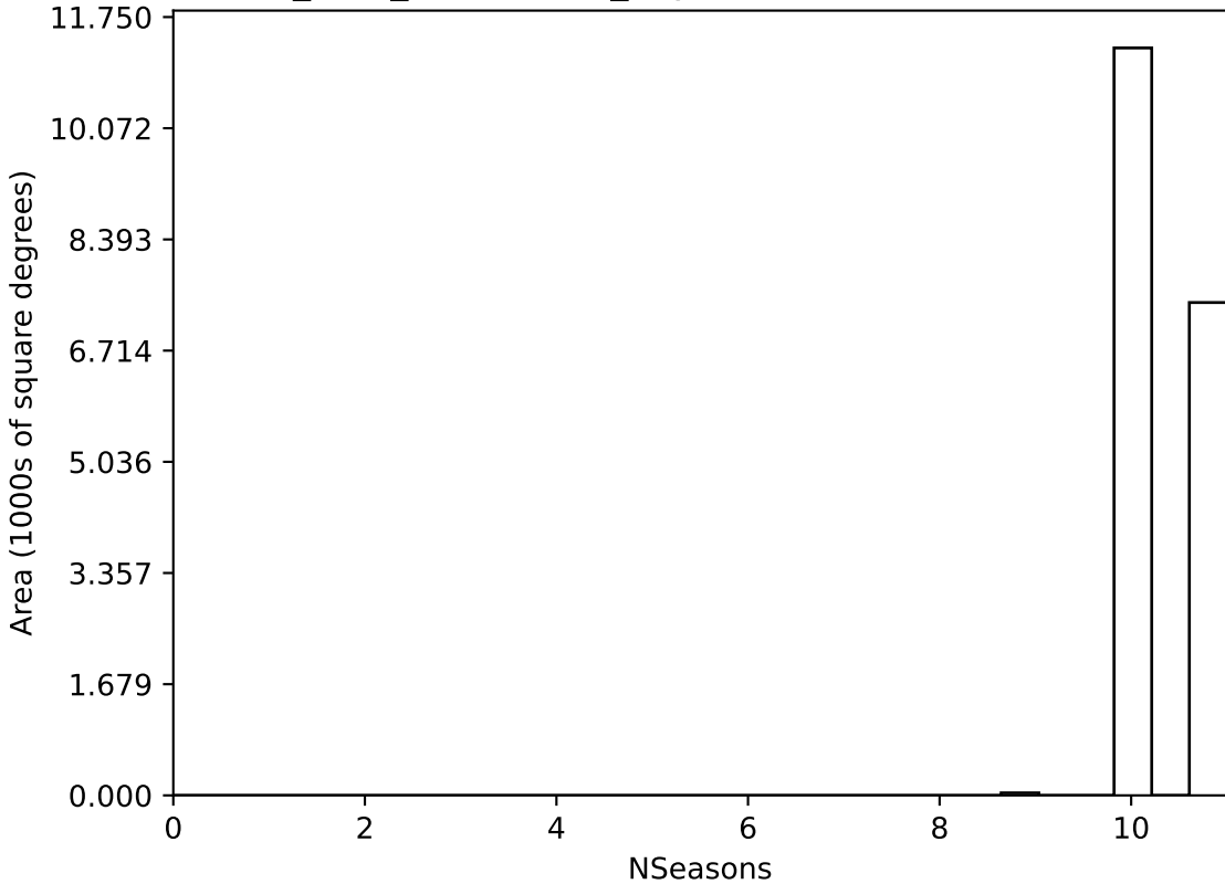
start_date_do-180v3.4_10yrs WFD all bands: NSeasons
