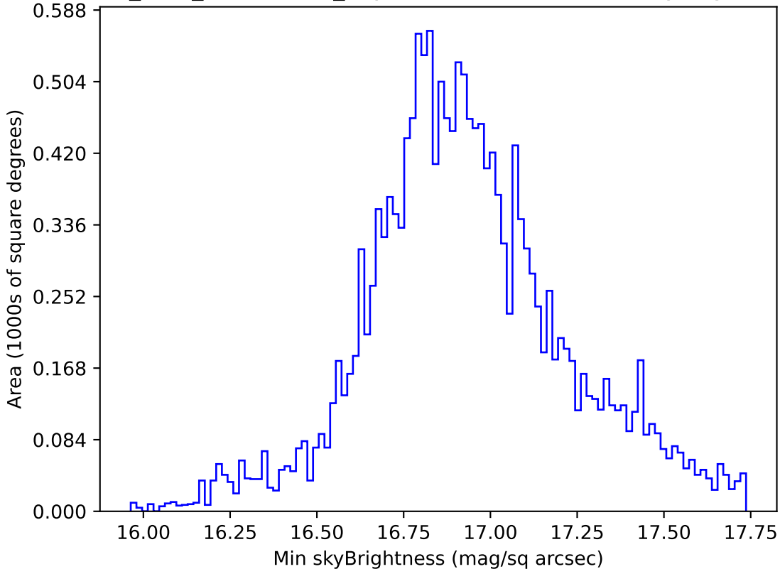
start_date_do-180v3.4_10yrs WFD all bands: Min skyBrightness
