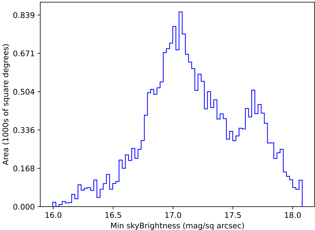
start_date_do-180v3.4_10yrs All sky y band: Min skyBrightness
