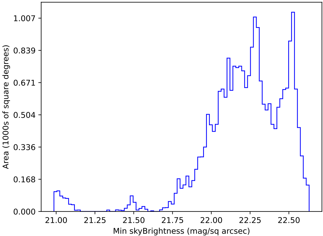
start_date_do-180v3.4_10yrs All sky u band: Min skyBrightness
