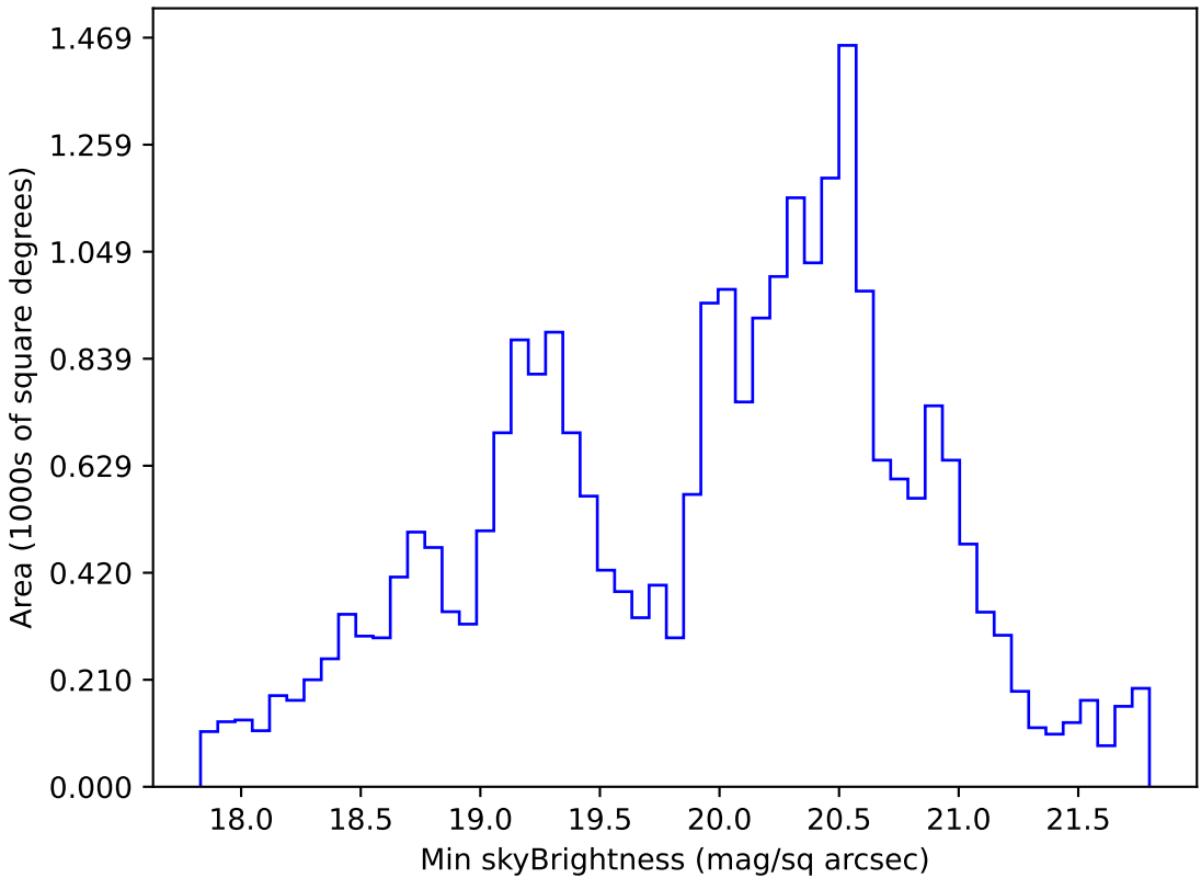
start_date_do-180v3.4_10yrs All sky g band: Min skyBrightness
