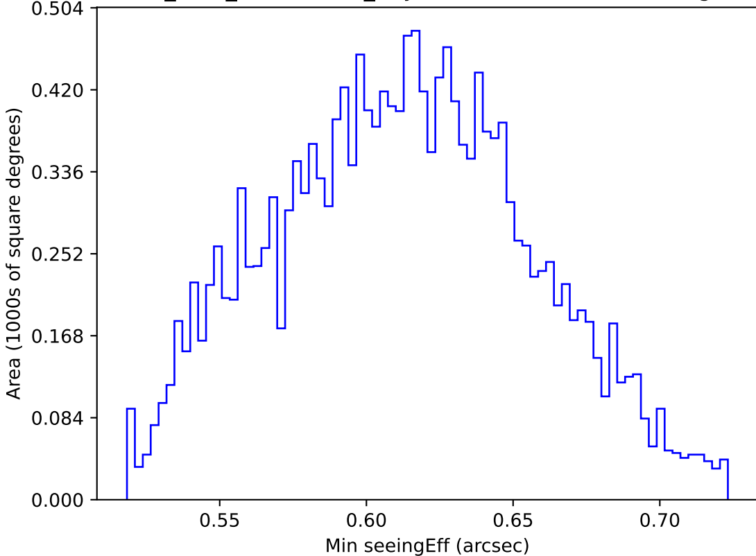
start_date_do-180v3.4_10yrs WFD z band: Min seeingEff
