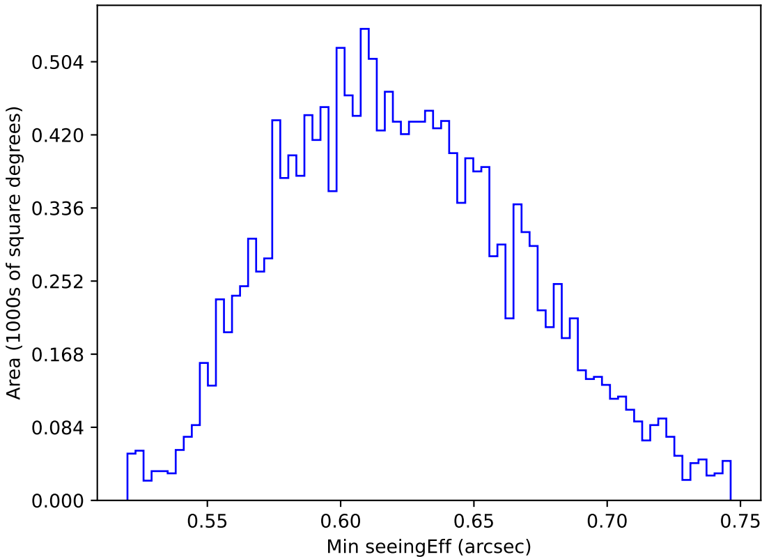
start_date_do-180v3.4_10yrs WFD y band: Min seeingEff
