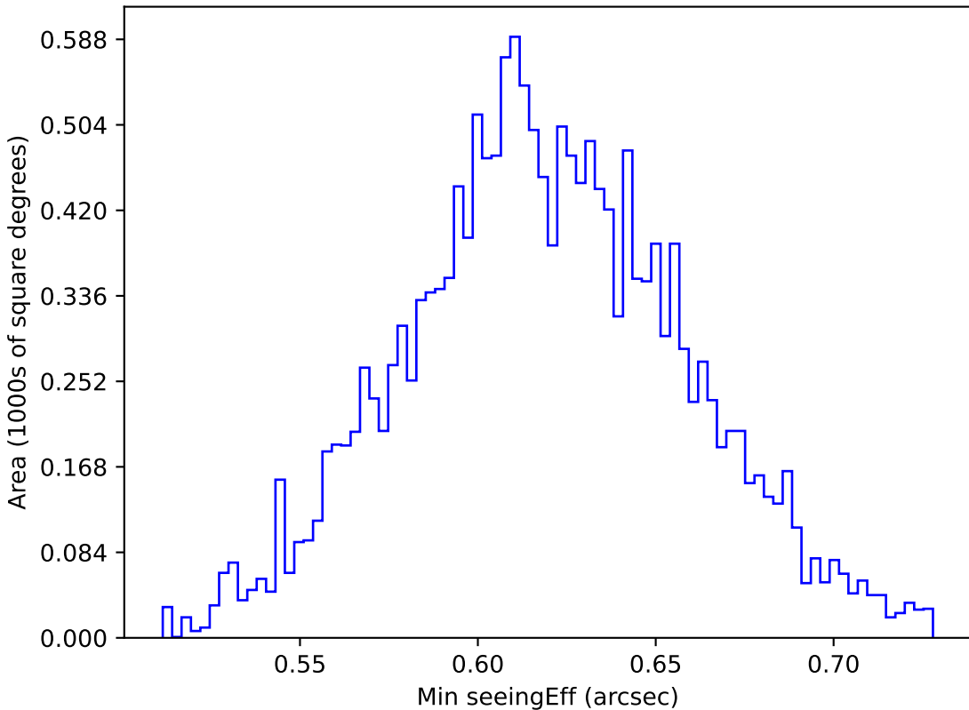
start_date_do-180v3.4_10yrs WFD r band: Min seeingEff
