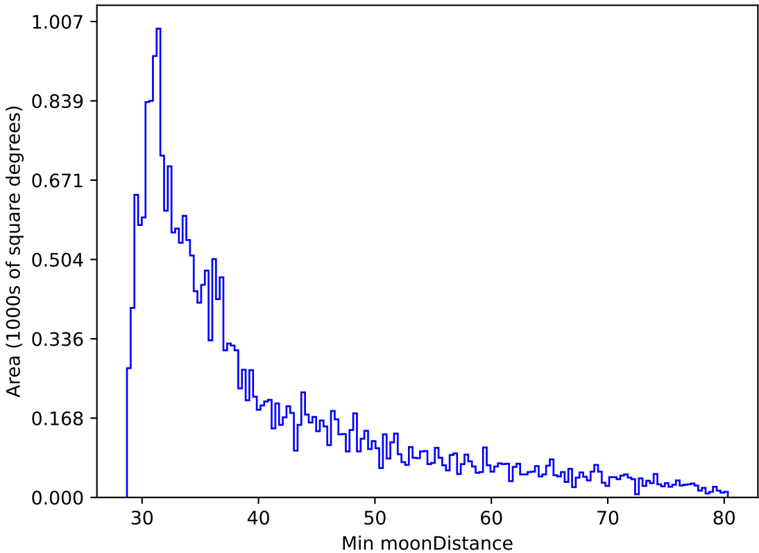
start_date_do-180v3.4_10yrs All sky r band: Min moonDistance
