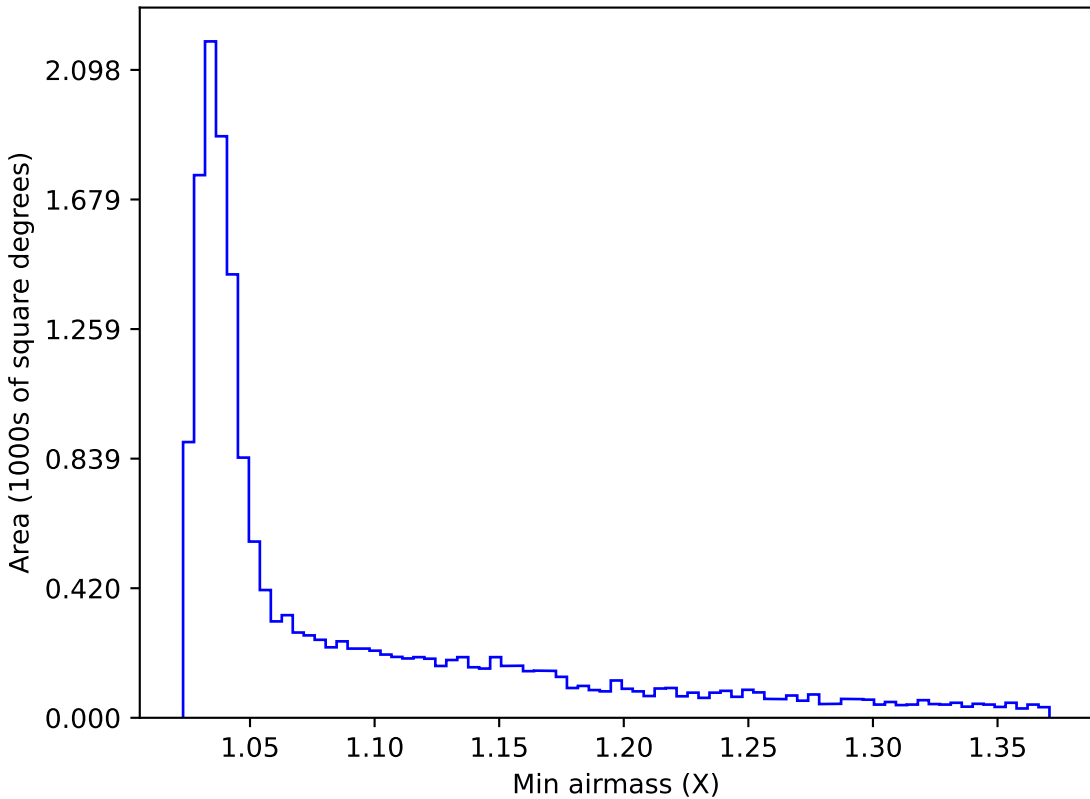
start_date_do-180v3.4_10yrs WFD g band: Min airmass
