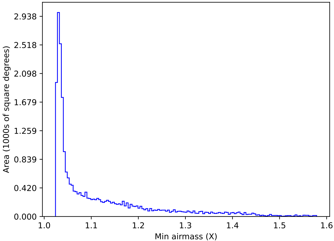
start_date_do-180v3.4_10yrs All sky y band: Min airmass
