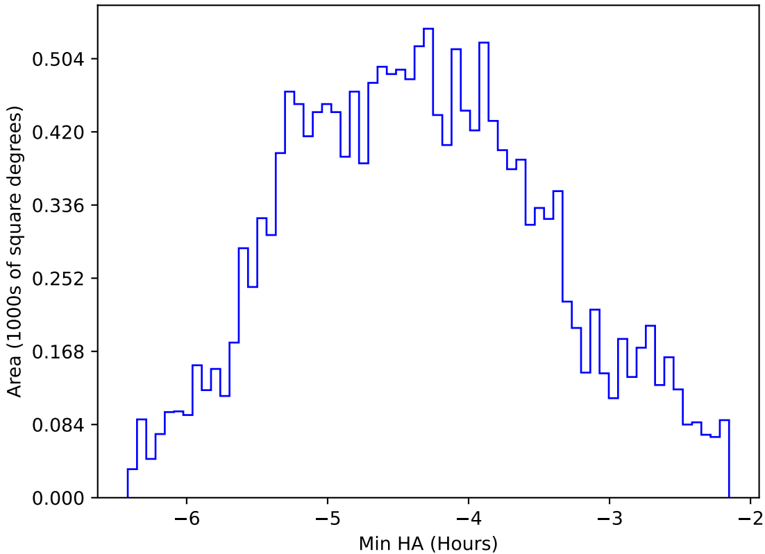
start_date_do-180v3.4_10yrs WFD z band: Min HA
