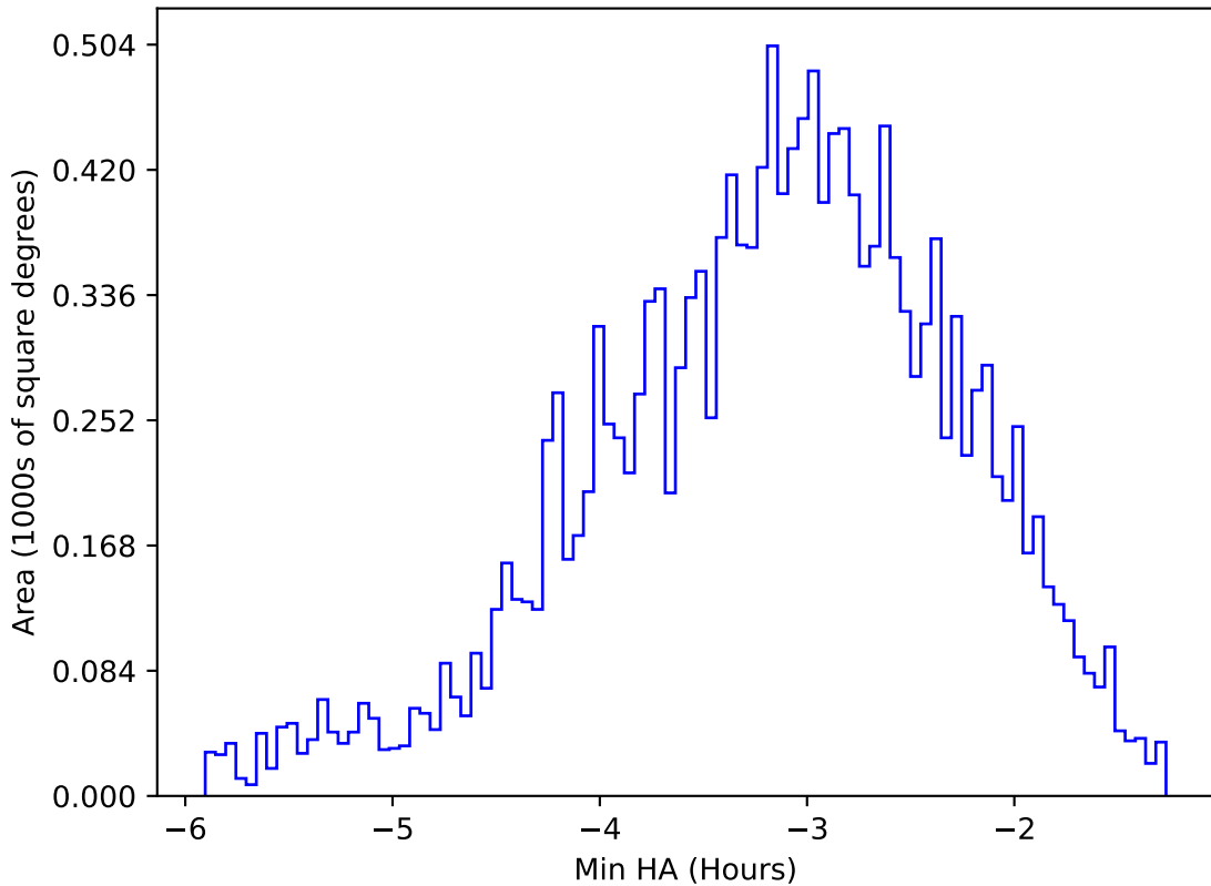
start_date_do-180v3.4_10yrs WFD u band: Min HA
