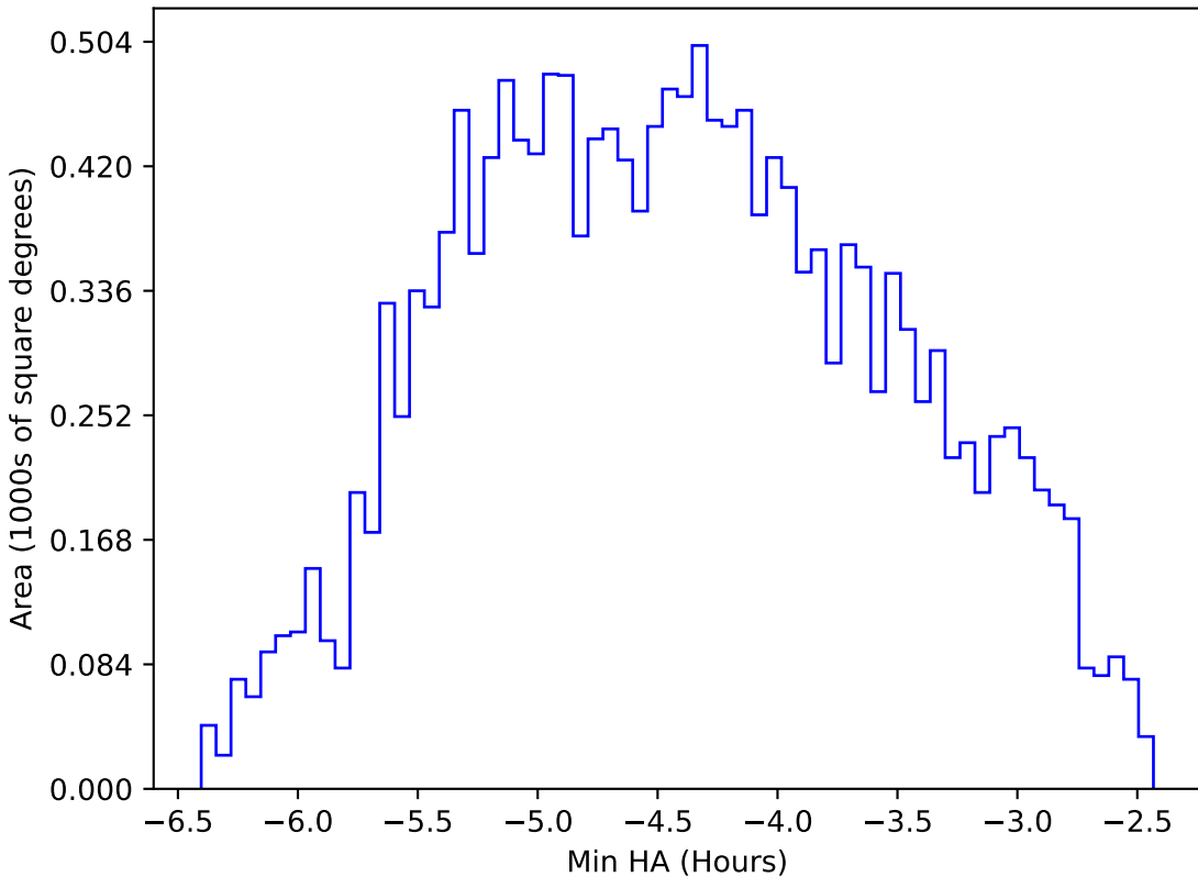
start_date_do-180v3.4_10yrs WFD r band: Min HA
