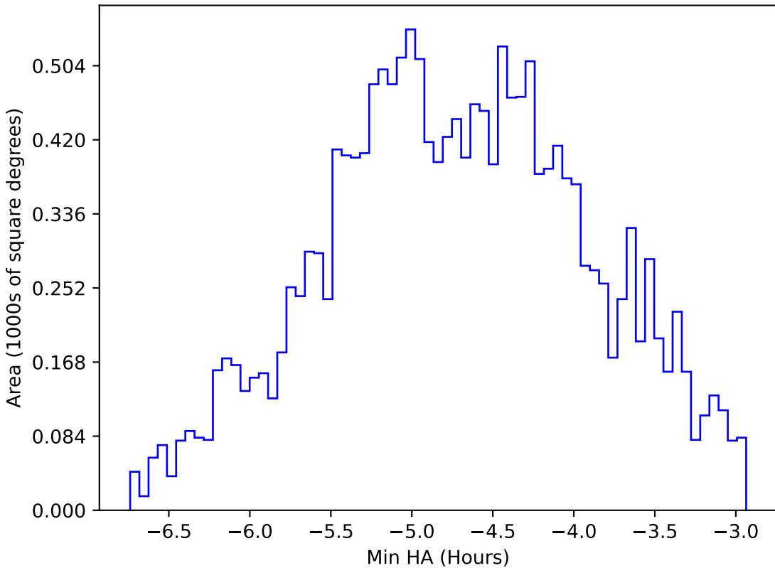
start_date_do-180v3.4_10yrs WFD all bands: Min HA
