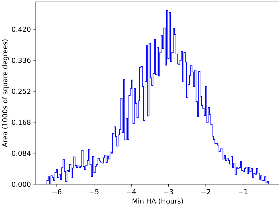
start_date_do-180v3.4_10yrs All sky u band: Min HA
