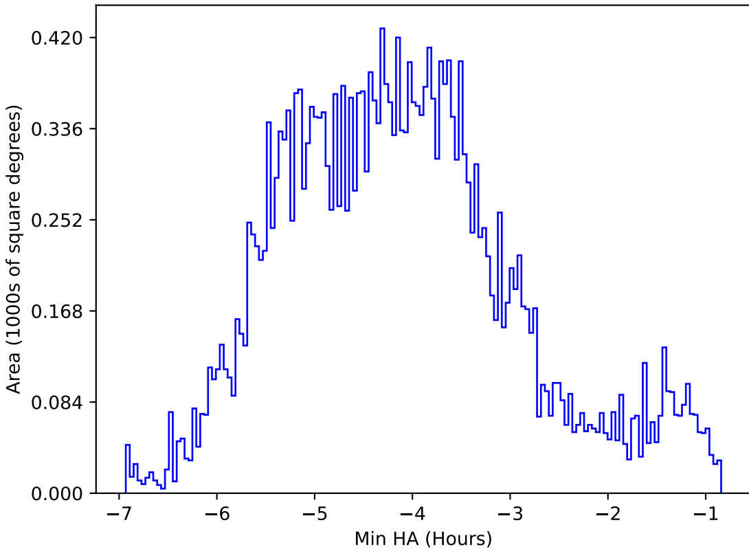
start_date_do-180v3.4_10yrs All sky r band: Min HA
