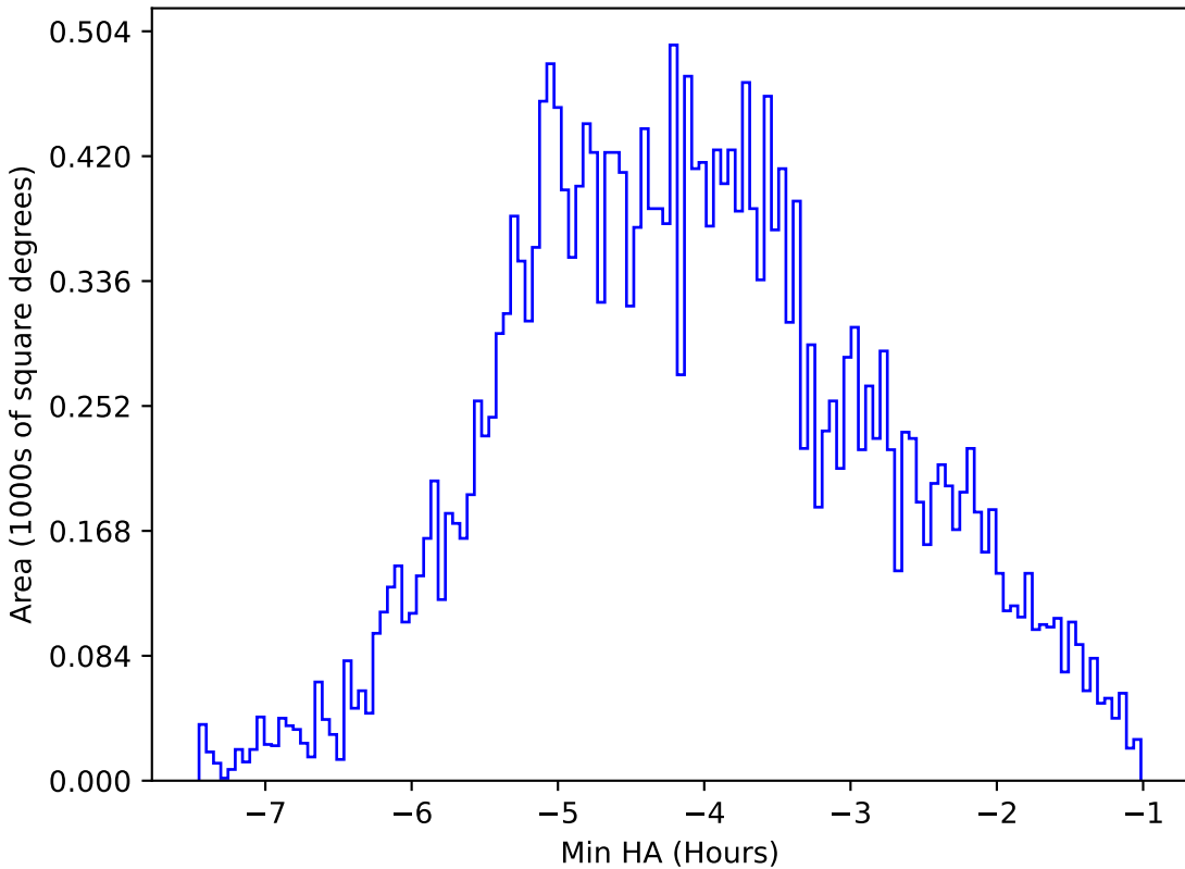
start_date_do-180v3.4_10yrs All sky i band: Min HA
