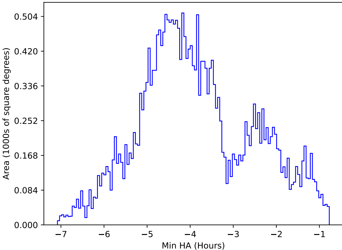
start_date_do-180v3.4_10yrs All sky g band: Min HA
