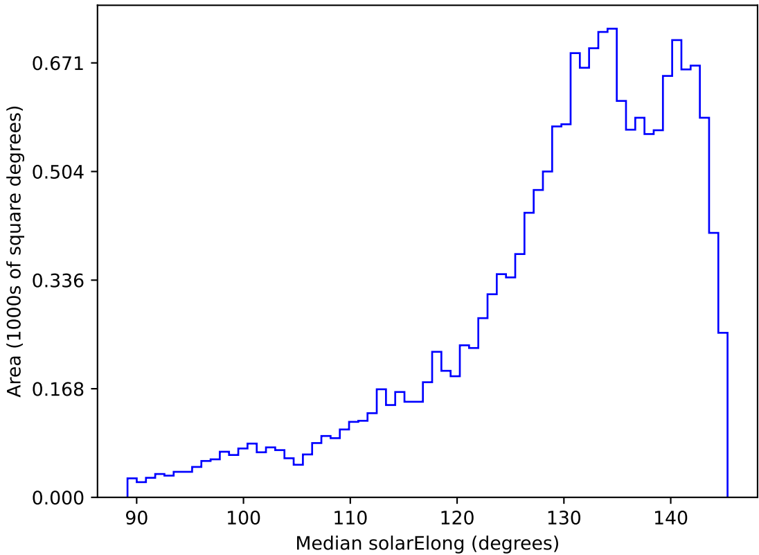
start_date_do-180v3.4_10yrs WFD all bands: Median solarElong
