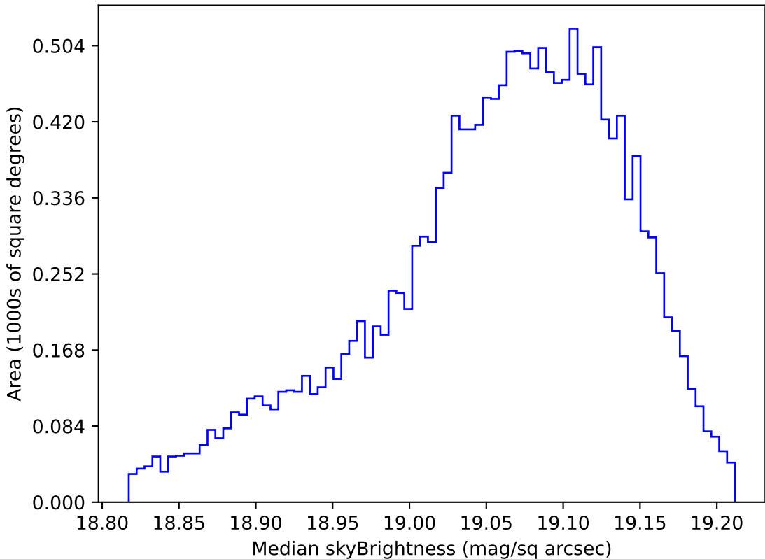
start_date_do-180v3.4_10yrs WFD z band: Median skyBrightness
