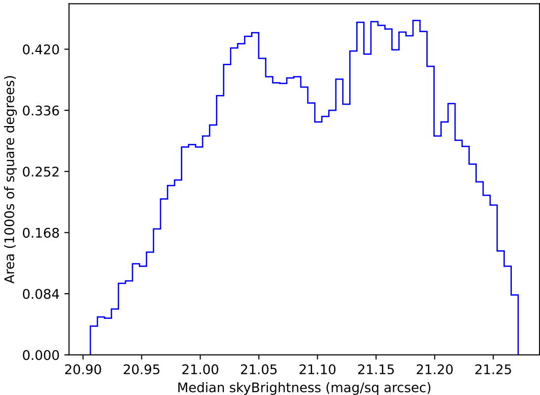
start_date_do-180v3.4_10yrs WFD r band: Median skyBrightness
