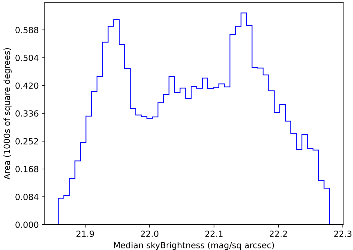
start_date_do-180v3.4_10yrs WFD g band: Median skyBrightness
