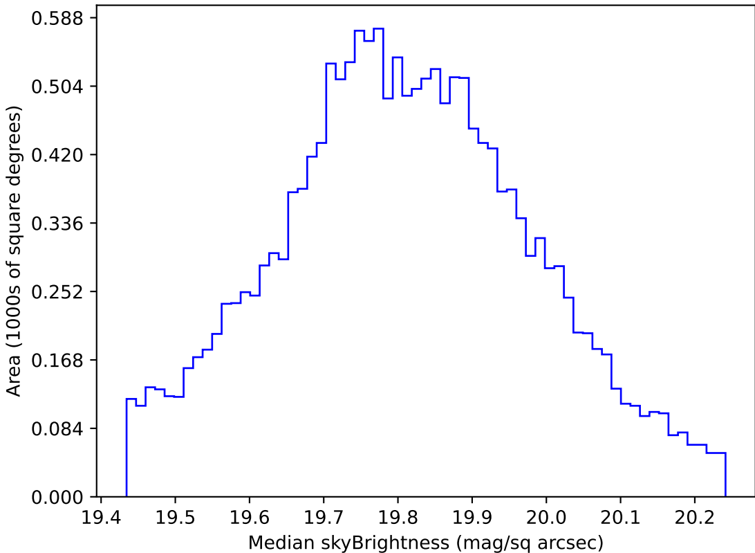
start_date_do-180v3.4_10yrs WFD all bands: Median skyBrightness
