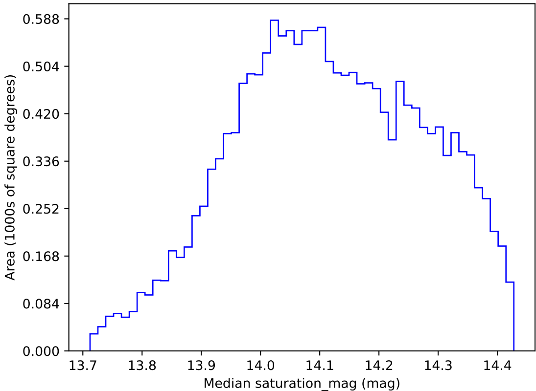
start_date_do-180v3.4_10yrs WFD z band: Median saturation_mag
