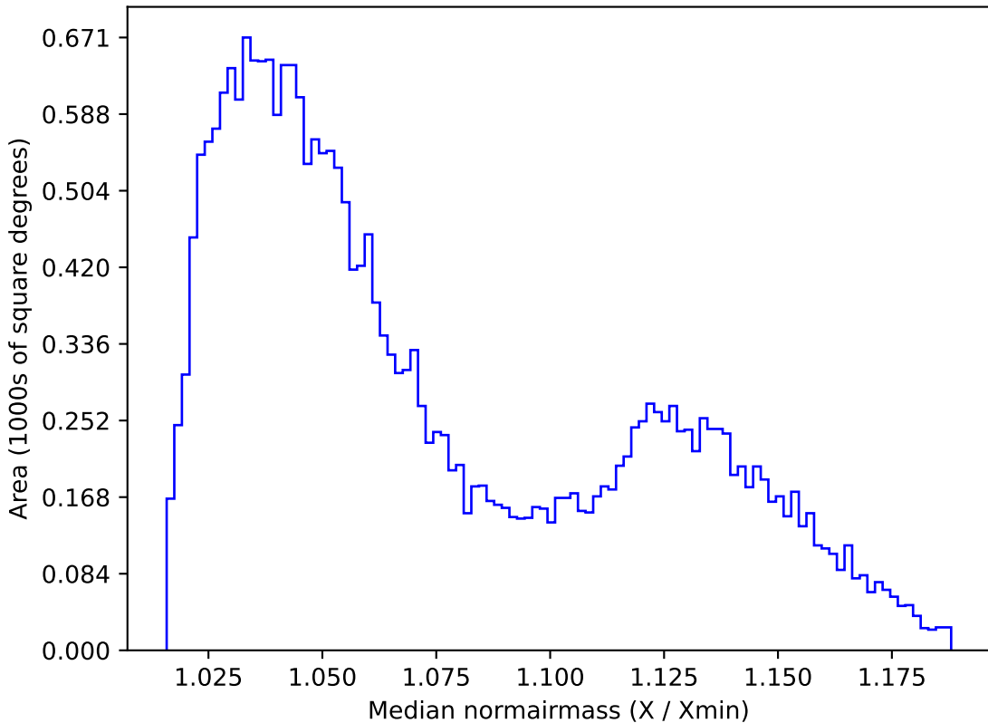
start_date_do-180v3.4_10yrs All sky i band: Median normairmass
