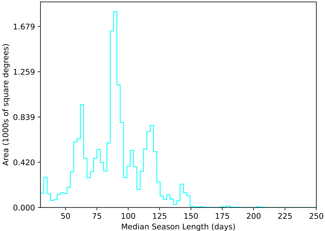
start_date_do-180v3.4_10yrs WFD u band: Median Season Length
