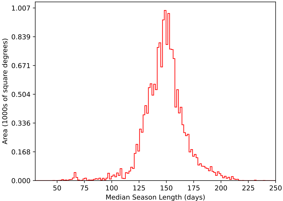
start_date_do-180v3.4_10yrs WFD i band: Median Season Length
