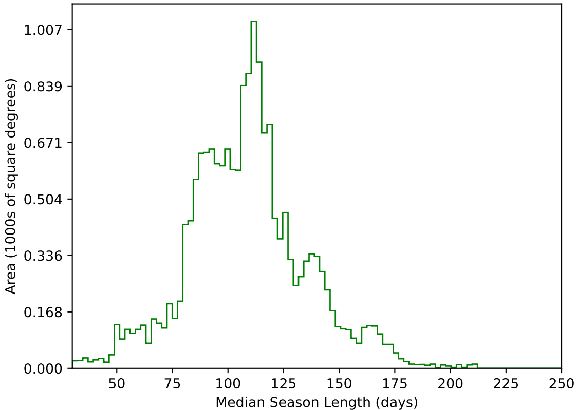
start_date_do-180v3.4_10yrs WFD g band: Median Season Length
