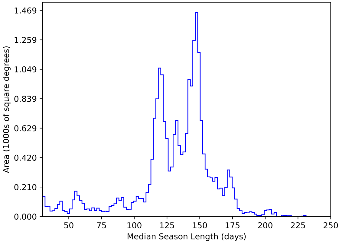
start_date_do-180v3.4_10yrs All sky y band: Median Season Length
