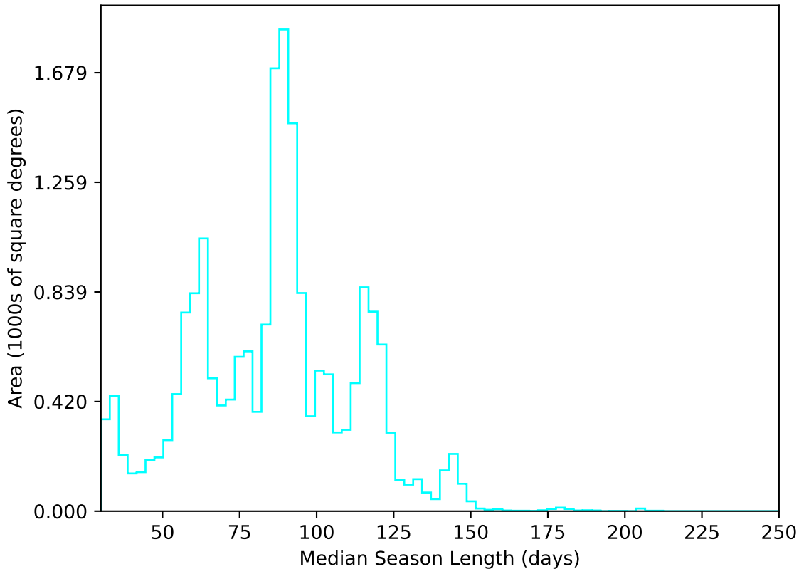
start_date_do-180v3.4_10yrs All sky u band: Median Season Length
