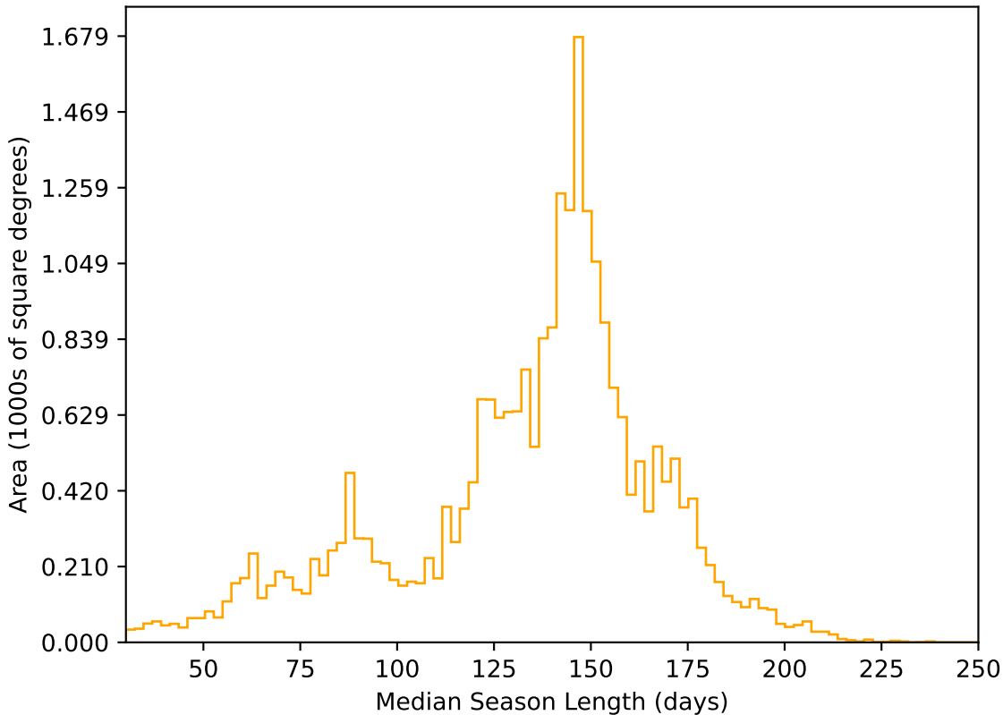
start_date_do-180v3.4_10yrs All sky r band: Median Season Length
