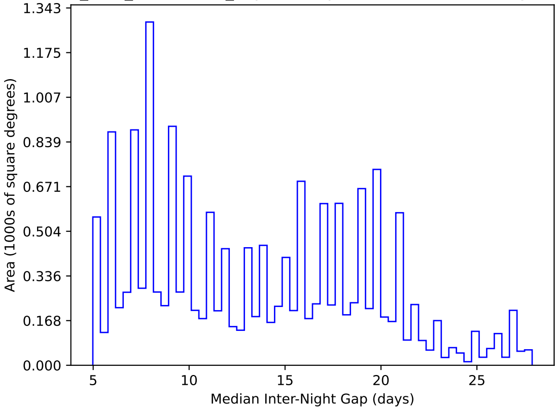
start_date_do-180v3.4_10yrs WFD y band: Median Inter-Night Gap
