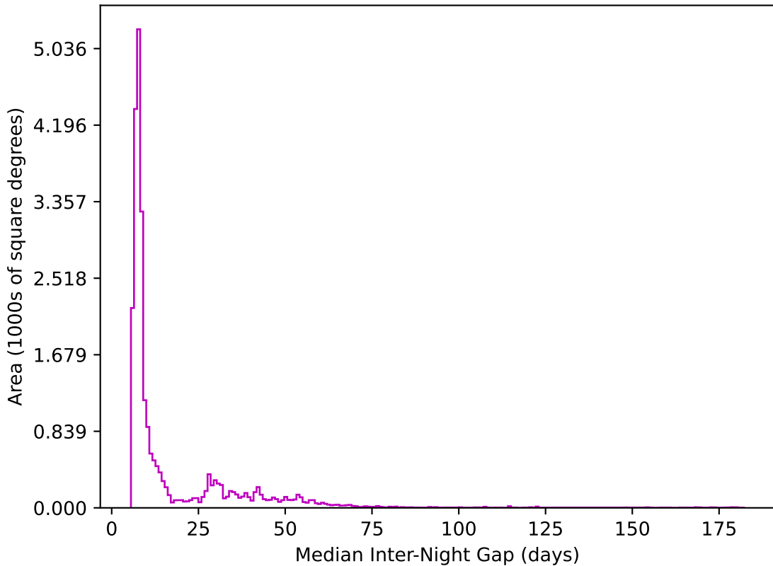
start_date_do-180v3.4_10yrs All sky z band: Median Inter-Night Gap
