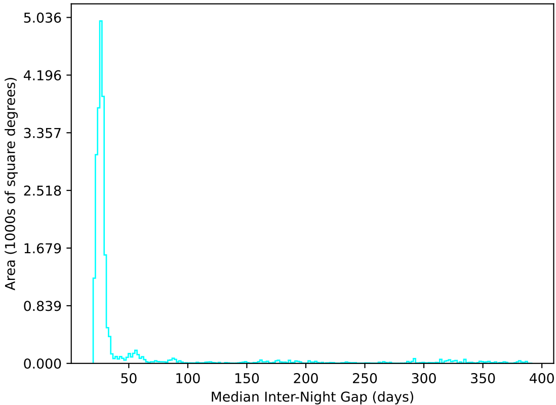
start_date_do-180v3.4_10yrs All sky u band: Median Inter-Night Gap
