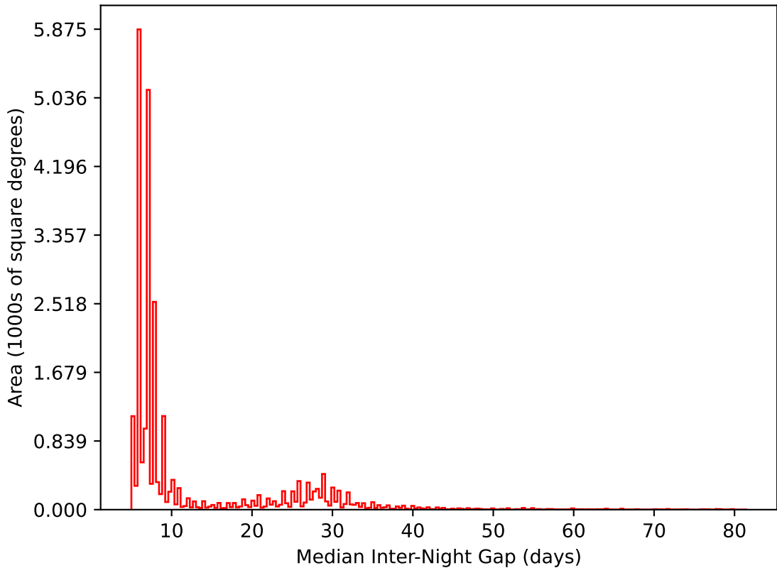
start_date_do-180v3.4_10yrs All sky i band: Median Inter-Night Gap
