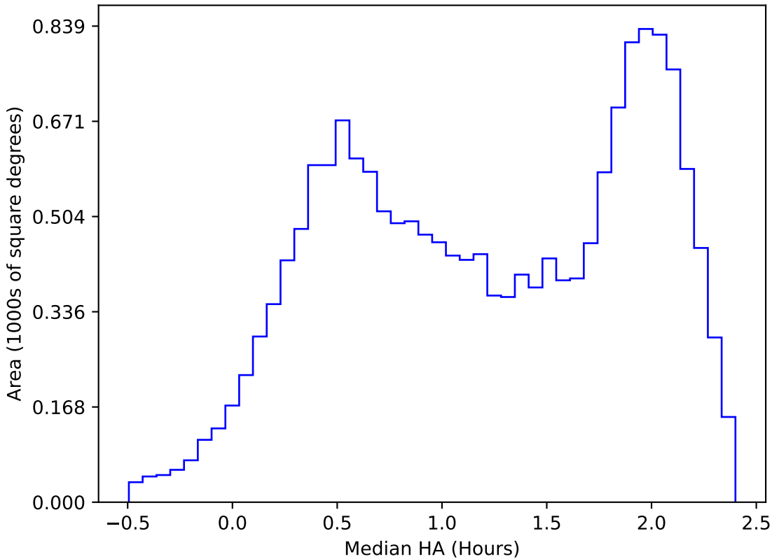
start_date_do-180v3.4_10yrs WFD z band: Median HA
