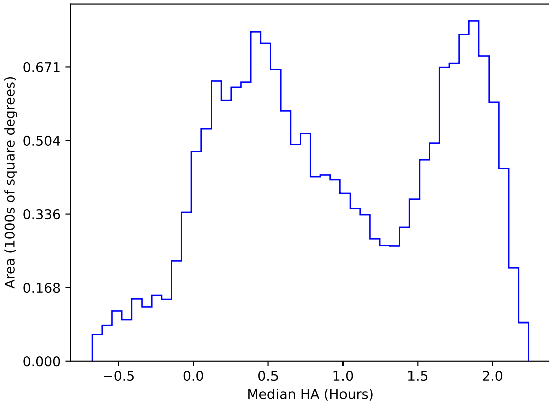
start_date_do-180v3.4_10yrs WFD r band: Median HA
