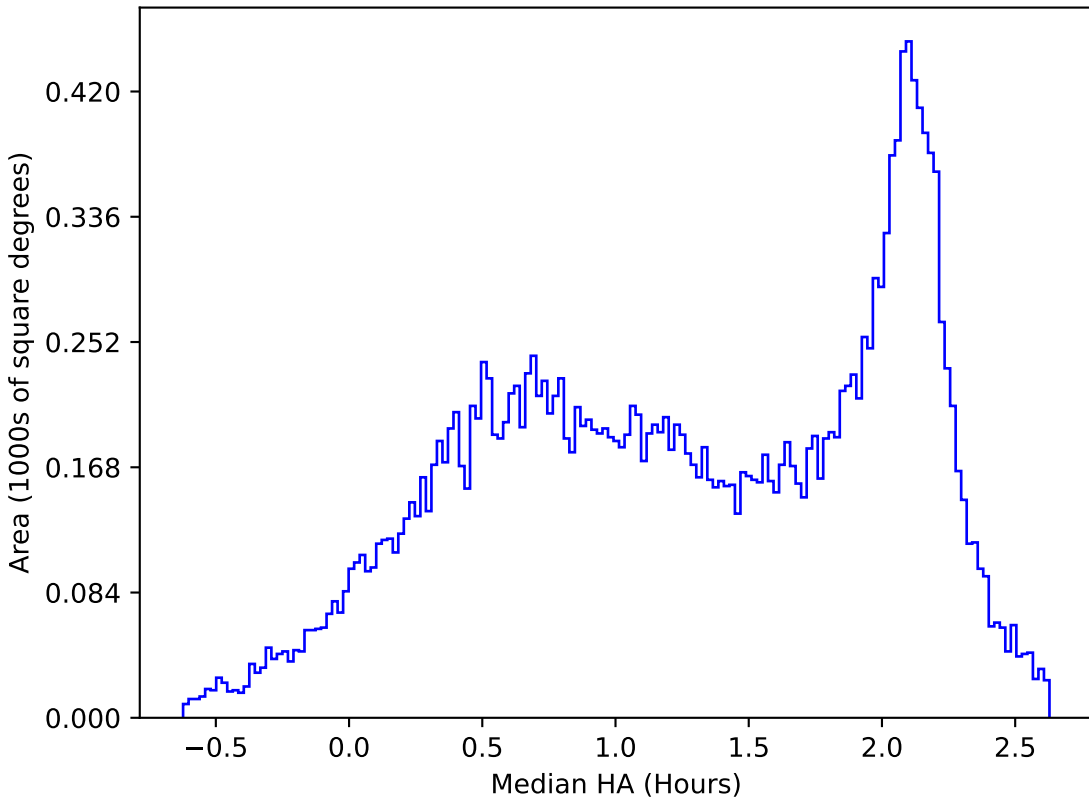
start_date_do-180v3.4_10yrs All sky y band: Median HA
